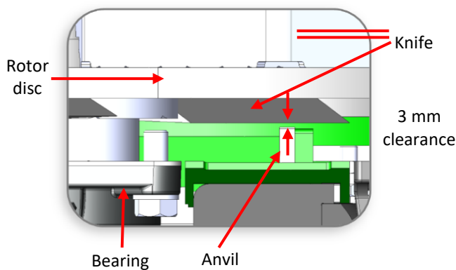
Top view: Knife and anvil set-up
