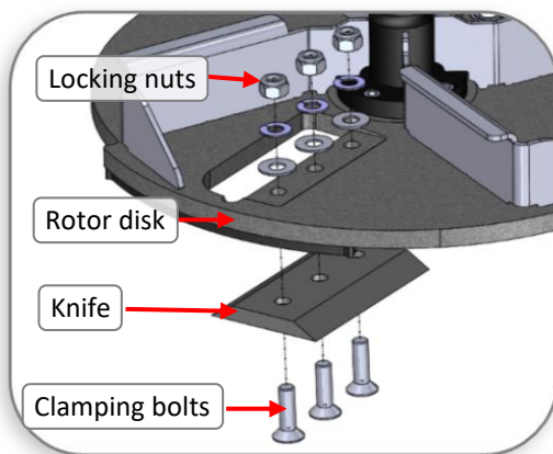
Side view: Cutting rotor
