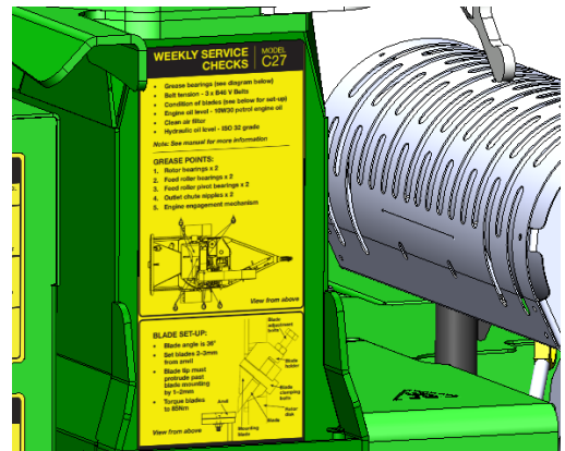
Rotor cover back
